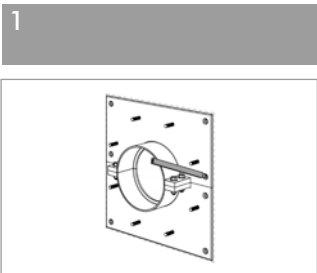
1 Position the divided casing pipe mounted together on the wall and mark the dowel holes.
