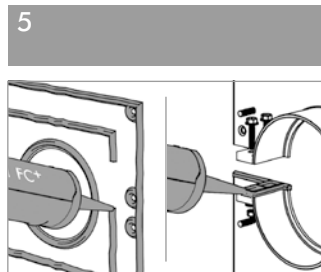
5 Apply the SikaFlex®-11 FC Purform® sealing adhesive (HDK) to the wall. Apply HDK in the area of the steel casing pipe to the wall and the dividing plates in a spider-web fashion. Screw the steel casing pipe halves together with mounting set. A prerequisite for a permanent sealing is the continuous webbing of the HDK.
