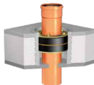
Variant: Curaflex® 3000 and Curaflex® C as bottom feed-through
